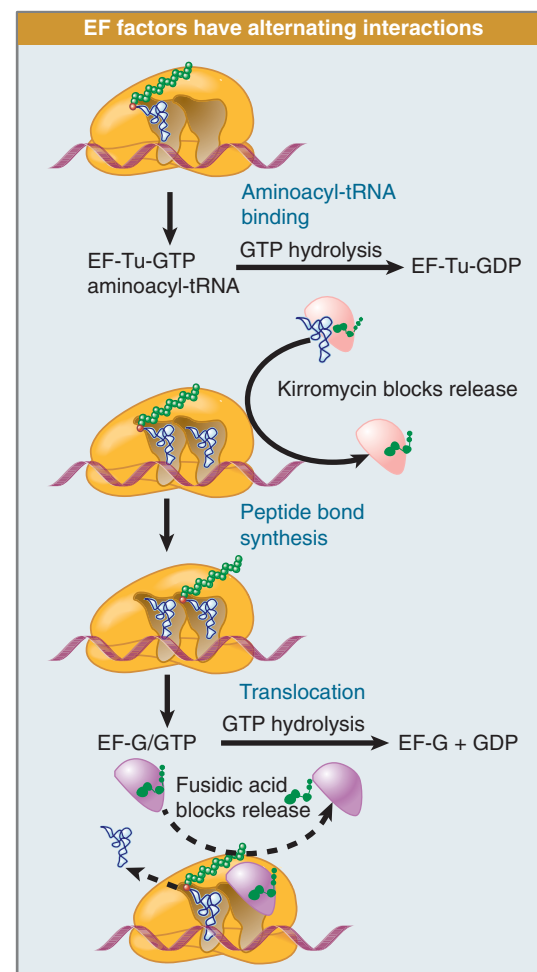
FIGURE 8.31 Binding of factors EF-Tu and EF-G alternates as ribosomes accept new aminoacyl-tRNA, form peptide bonds, and translocate.
