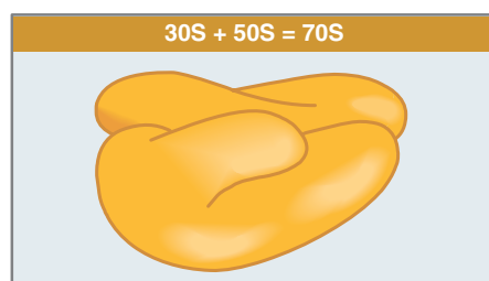
FIGURE 8.38 The platform of the 30S subunit fits into the notch of the 50S subunit to form the 70S ribosome.
