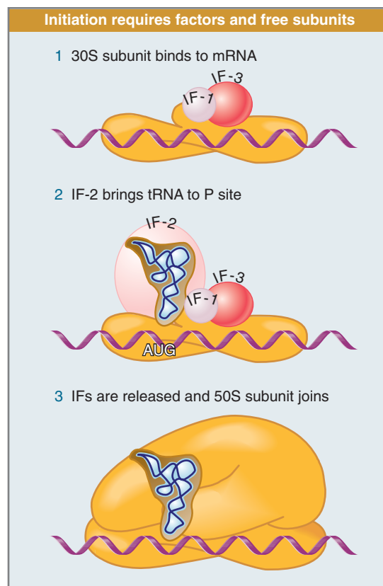
FIGURE 8.10 Initiation factors stabilize free 30S subunits and bind initiator tRNA to the 30S-mRNA complex.
