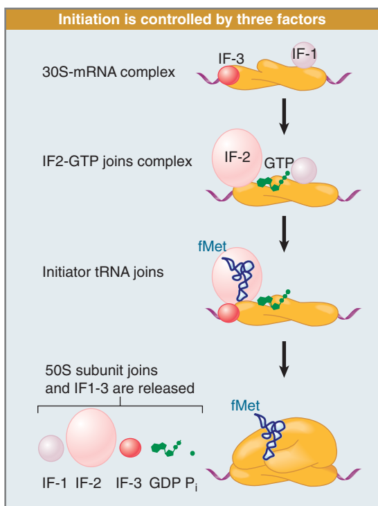
FIGURE 8.15 IF-2 is needed to bind fMet-tRNA f to the 30S-mRNA complex. After 50S binding, all IF factors are released and GTP is cleaved.
