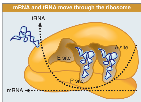
FIGURE 8.6 tRNA and mRNA move through the ribosome in the same direction.
