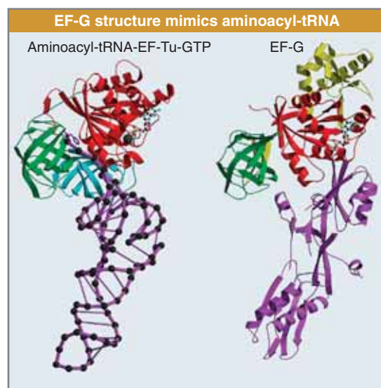
FIGURE 8.30 The structure of the ternary complex of aminoacyl-tRNA-EF-Tu-GTP (left) resembles the structure of EF-G (right). Structurally conserved domains of EF-Tu and EF-G are in red and green; the tRNA and the domain resembling it in EF-G are in purple. Photo courtesy of Poul Nissen, University of Aarhus, Denmark.
