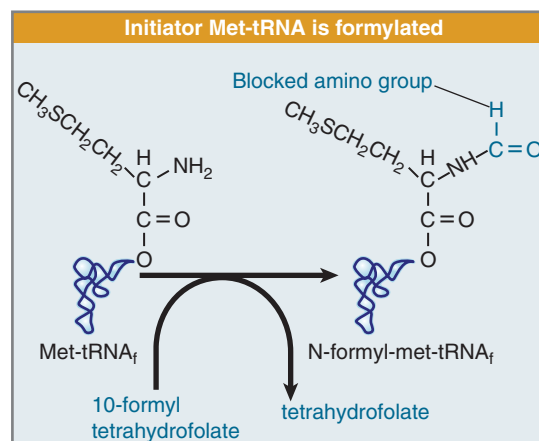
FIGURE 8.12 The initiator N-formyl-methionyl-tRNA (fMet-tRNA f ) is generated by formylation of methionyl-tRNA, using formyl-tetrahydrofolate as cofactor.
