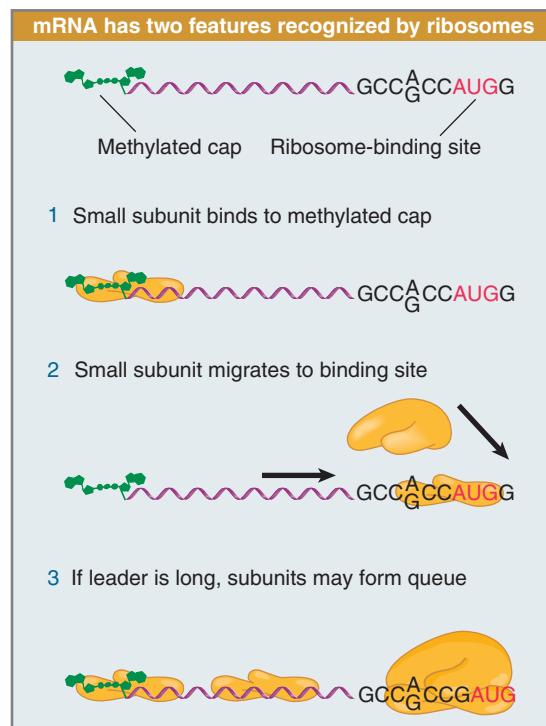
FIGURE 8.18 Eukaryotic ribosomes migrate from the 5' end of mRNA to the ribosome binding site, which includes an AUG initiation codon.
