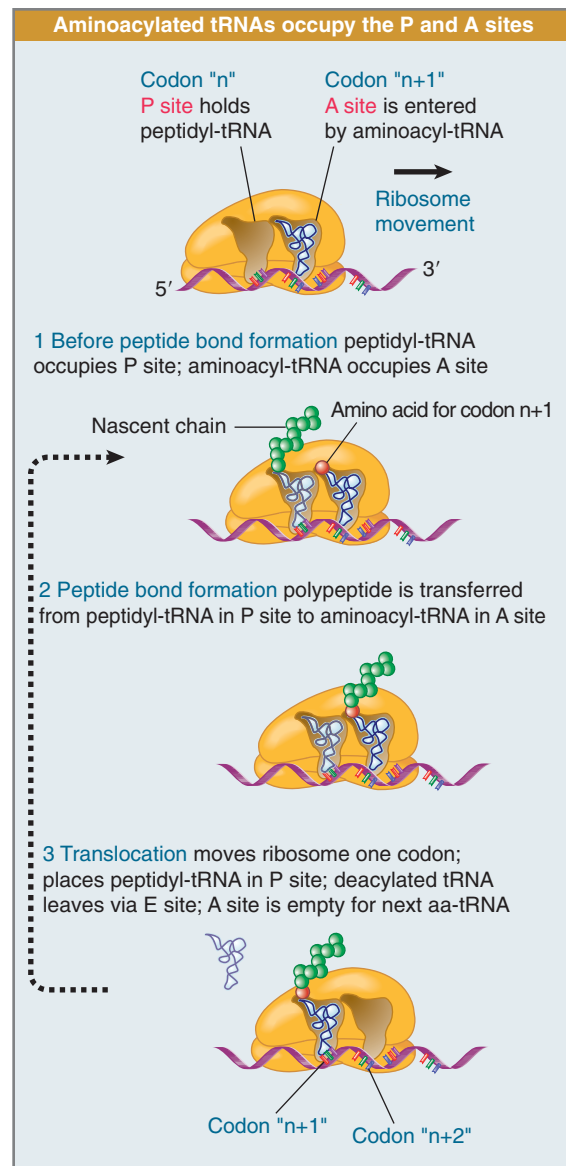
FIGURE 8.3 The ribosome has two sites for binding charged tRNA.
