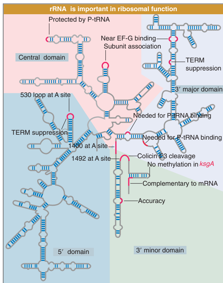
FIGURE 8.45 Some sites in 16S rRNA are protected from chemical probes when 50S subunits join 30S subunits or when aminoacyl-tRNA binds to the A site. Others are the sites of mutations that affect protein synthesis. TERM suppression sites may affect termination at some or several termination codons. The large colored blocks indicate the four domains of the rRNA.
