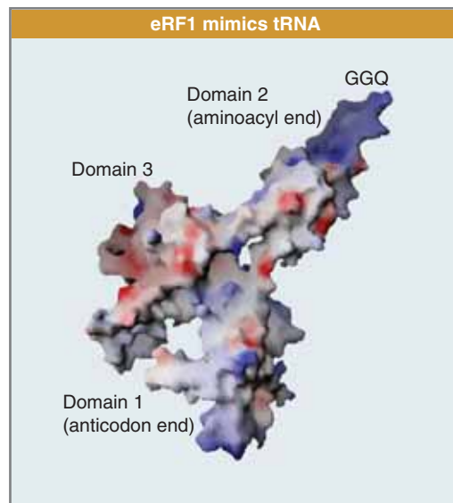
FIGURE 8.33 The eukaryotic termination factor eRF1 has a structure that mimics tRNA. The motif GGQ at the tip of domain 2 is essential for hydrolyzing the polypeptide chain from tRNA. Photo courtesy of David Barford, The Institute of Cancer Research.
