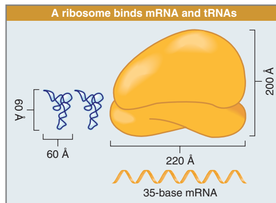
FIGURE 8.1 Size comparisons show that the ribosome is large enough to bind tRNAs and mRNA.
