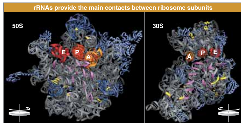
FIGURE 8.41 Contacts between the ribosomal subunits are mostly made by RNA (shown in purple). Contacts involving proteins are shown in yellow. The two subunits are rotated away from one another to show the faces where contacts are made; from a plane of contact perpendicular to the screen, the 50S subunit is rotated 90° counterclockwise, and the 30S is rotated 90° clockwise (this shows it in the reverse of the usual orientation). Photo courtesy of Harry Noller, University of California, Santa Cruz.
