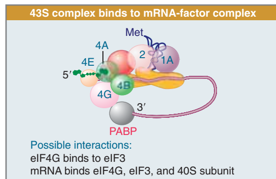
FIGURE 8.23 Interactions involving initiation factors are important when mRNA binds to the 43S complex.
