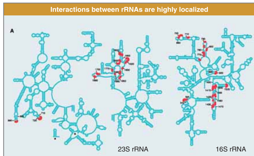
FIGURE 8.40 Contact points between the rRNAs are located in two domains of 16S rRNA and one domain of 23S rRNA. Photo courtesy of Harry Noller, University of California, Santa Cruz.
