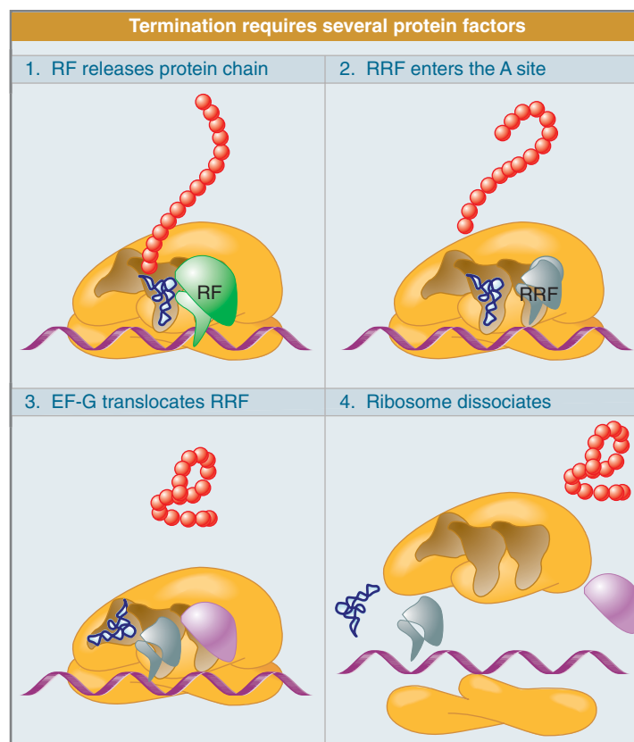
FIGURE 8.35 The RF (release factor) terminates protein synthesis by releasing the protein chain. The RRF (ribosome recycling factor) releases the last tRNA, and EF-G releases RRF, causing the ribosome to dissociate.
