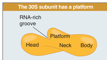
FIGURE 8.36 The 30S subunit has a head separated by a neck from the body, with a protruding platform.
