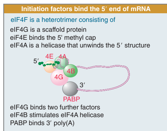
FIGURE 8.20 The heterotrimer eIF4F binds the 5' end of mRNA and also binds further factors.
