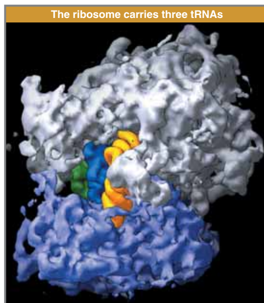
FIGURE 8.42 The 70S ribosome consists of the 50S subunit (white) and the 30S subunit (purple) with three tRNAs located superficially: yellow in the A site, blue in the P site, and green in the E site. Photo courtesy of Harry Noller, University of California, Santa Cruz.
