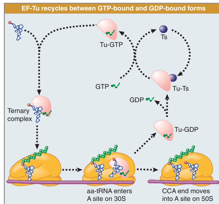
FIGURE 8.25 EF-Tu-GTP places aminoacyl-tRNA on the ribosome and then is released as EF-Tu-GDP. EF-Ts is required to mediate the replacement of GDP by GTP. The reaction consumes GTP and releases GDP. The only aminoacyl-tRNA that cannot be recognized by EF-Tu-GTP is fMet-tRNA f , whose failure to bind prevents it from responding to internal AUG or GUG codons.
