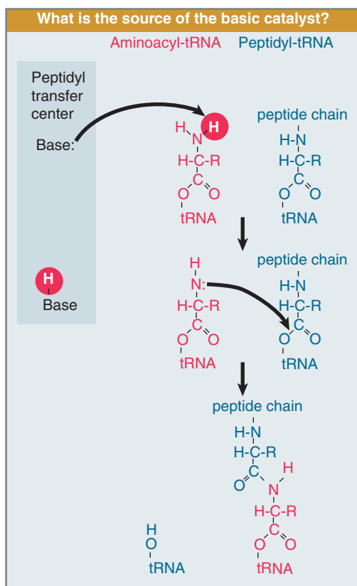
FIGURE 8.48 Peptide bond formation requires acid-base catalysis in which an H atom is transferred to a basic residue.
