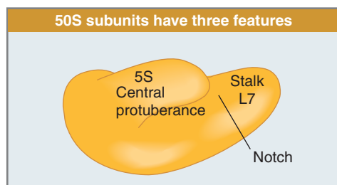
FIGURE 8.37 The 50S subunit has a central protuberance where 5S rRNA is located, separated by a notch from a stalk made of copies of the protein L7.
