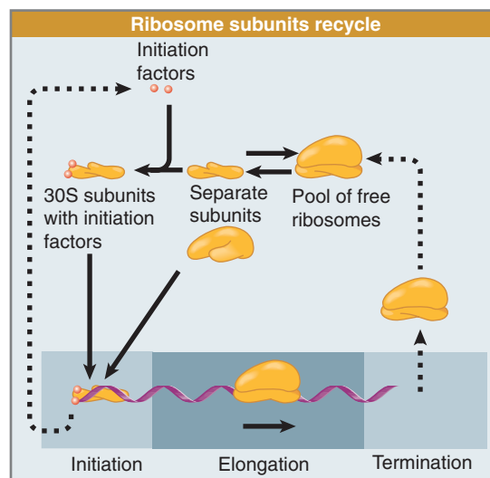
FIGURE 8.9 Initiation requires free ribosome subunits. When ribosomes are released at termination, the 30S subunits bind initiation factors and dissociate to generate free subunits. When subunits reassociate to give a functional ribosome at initiation, they release the factors.
