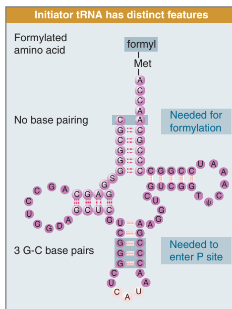
FIGURE 8.13 fMet-tRNA f has unique features that distinguish it as the initiator tRNA.
