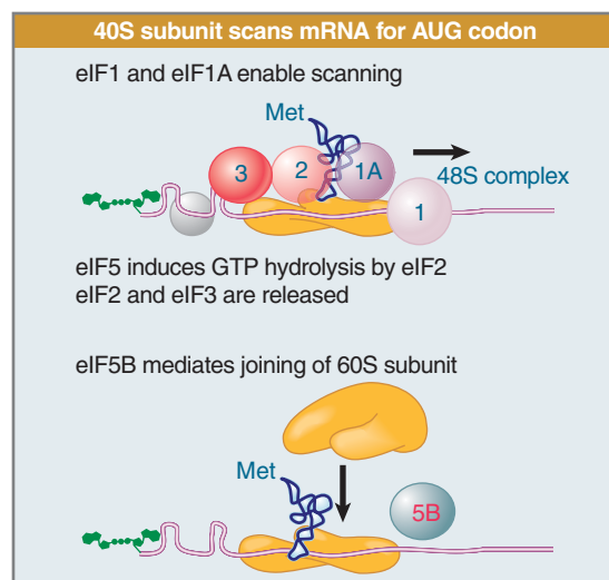
FIGURE 8.24 eIF1 and eIF1A help the 43S initiation complex to scan the mRNA until it reaches an AUG codon. eIF2 hydrolyzes its GTP to enable its release together with eIF3. eIF5B mediates 60S–40S joining.
