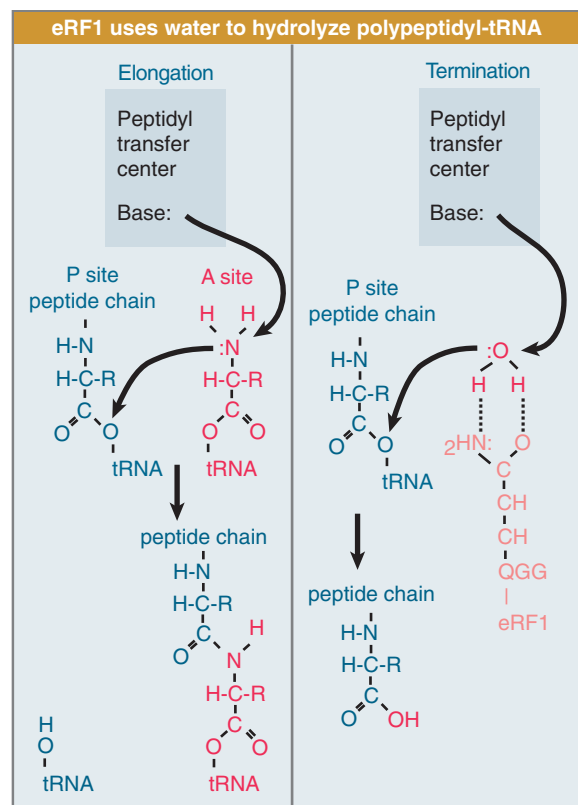
FIGURE 8.34 Peptide transfer and termination are similar reactions in which a base in the peptidyl transfer center triggers a transesterification reaction by attacking an N-H or O-H bond, releasing the N or O to attack the link to tRNA.
