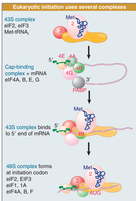
FIGURE 8.19 Some initiation factors bind to the 40S ribosome subunit to form the 43S complex; others bind to mRNA. When the 43S complex binds to mRNA, it scans for the initiation codon and can be isolated as the 48S complex.
