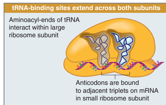
FIGURE 8.4 The P and A sites position the two interacting tRNAs across both ribosome subunits.
