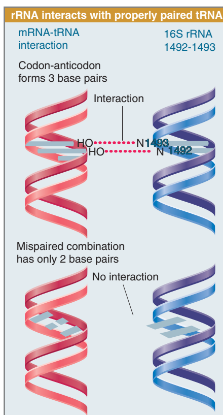
FIGURE 8.47 Codon-anticodon pairing supports interaction with adenines 1492–1493 of 16S rRNA, but mispaired tRNA-mRNA cannot interact.
