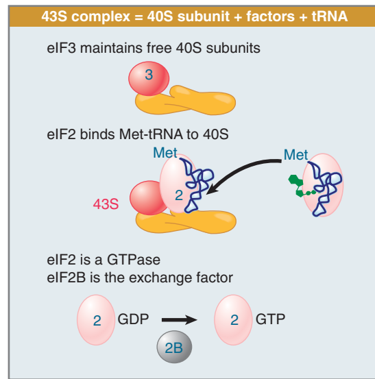
FIGURE 8.22 Initiation factors bind the initiator Met-tRNA to the 40S subunit to form a 43S complex. Later in the reaction, GTP is hydrolyzed when eIF-2 is released in the form of eIF2-GDP. eIF-2B regenerates the active form.
