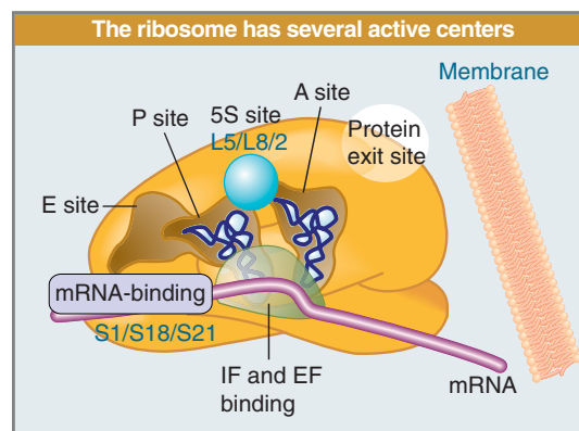
FIGURE 8.44 The ribosome has several active centers. It may be associated with a membrane. mRNA takes a turn as it passes through the A and P sites, which are angled with regard to each other. The E site lies beyond the P site. The peptidyl transferase site (not shown) stretches across the tops of the A and P sites. Part of the site bound by EF-Tu/G lies at the base of the A and P sites.
