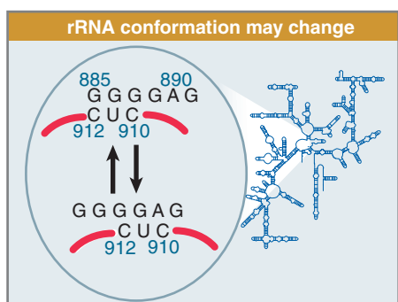
FIGURE 8.46 A change in conformation of 16S rRNA may occur during protein synthesis.
