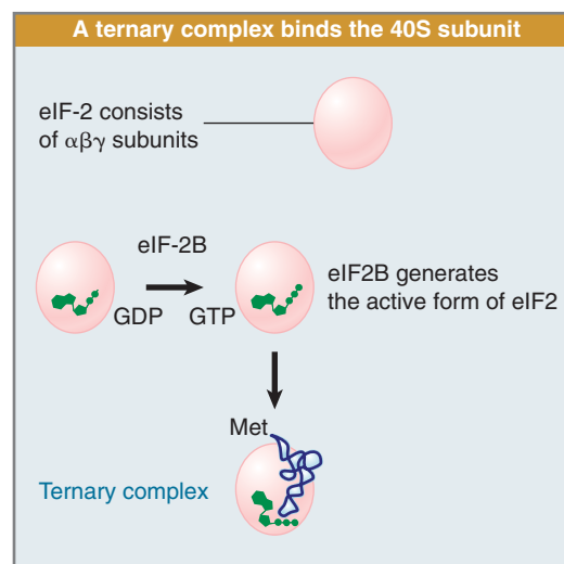
FIGURE 8.21 In eukaryotic initiation, eIF-2 forms a ternary complex with Met-tRNA i . The ternary complex binds to free 40S subunits, which attach to the 5' end of mRNA. Later in the reaction, GTP is hydrolyzed when eIF-2 is released in the form of eIF2-GDP. eIF-2B regenerates the active form.
