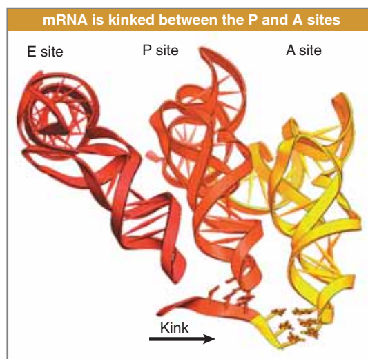
FIGURE 8.43 Three tRNAs have different orientations on the ribosome. mRNA turns between the P and A sites to allow aminoacyl-tRNAs to bind adjacent codons. Photo courtesy of Harry Noller, University of California, Santa Cruz.
