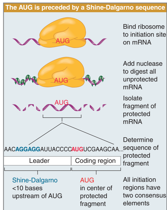
FIGURE 8.16 Ribosome-binding sites on mRNA can be recovered from initiation complexes. They include the upstream Shine-Dalgarno sequence and the initiation codon.
