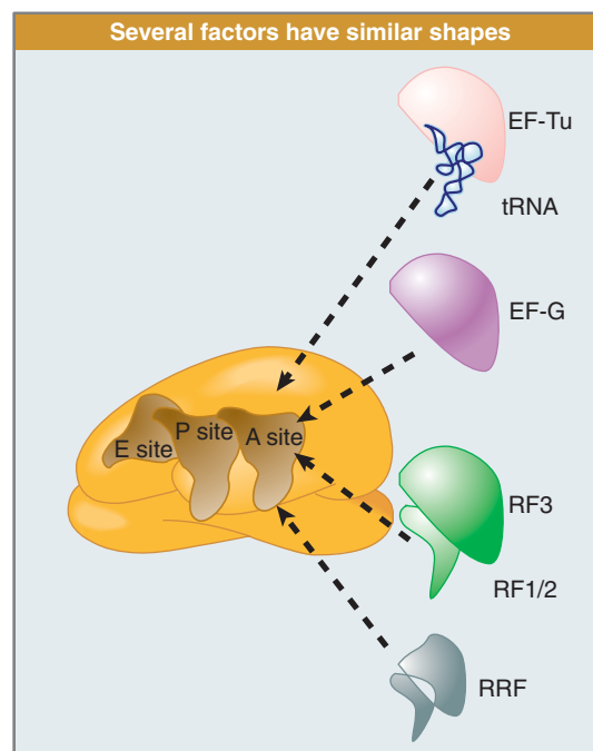
FIGURE 8.32 Molecular mimicry enables the elongation factor Tu-tRNA complex, the translocation factor EF-G, and the release factors RF1/2-RF3 to bind to the same ribosomal site. RRF is the ribosome recycling factor (see Figure 8.35)
