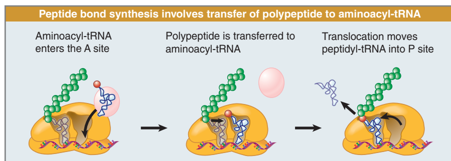
FIGURE 8.5 Aminoacyl-tRNA enters the A site, receives the polypeptide chain from peptidyl-tRNA, and is transferred into the P site for the next cycle of elongation.
