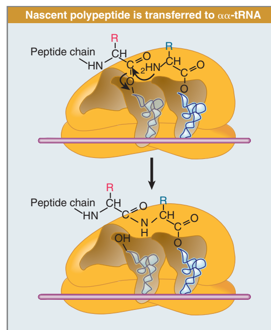
FIGURE 8.26 Peptide bond formation takes place by reaction between the polypeptide of peptidyl-tRNA in the P site and the amino acid of aminoacyl-tRNA in the A site.
