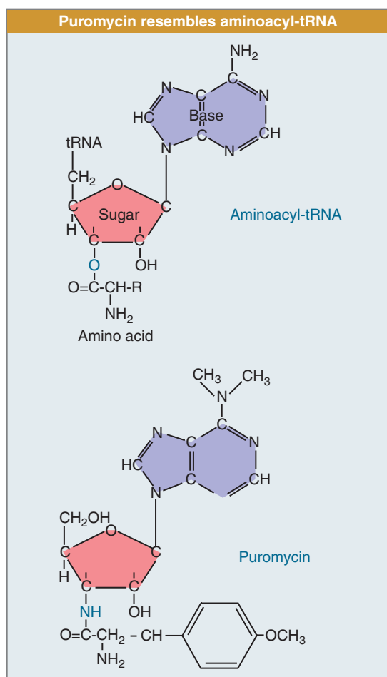
FIGURE 8.27 Puromycin mimics aminoacyl-tRNA because it resembles an aromatic amino acid linked to a sugar-base moiety.
