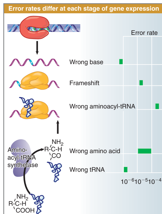
FIGURE 8.8 Errors occur at rates from 10^{-6} to 5 \times 10^{-4} at different stages of protein synthesis.
