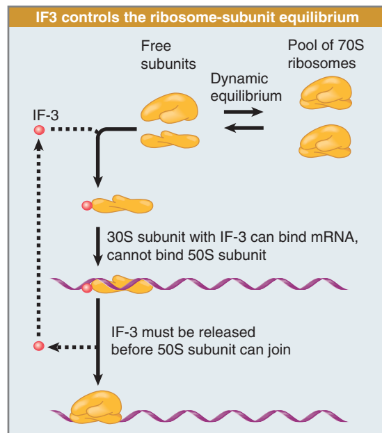
FIGURE 8.11 Initiation requires 30S subunits that carry IF-3.
