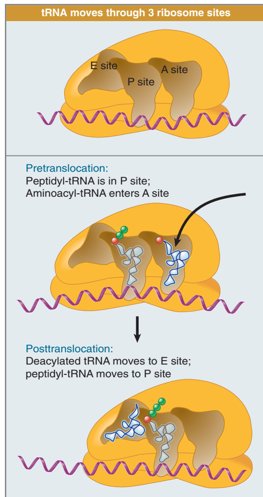
FIGURE 8.28 A bacterial ribosome has three tRNA-binding sites. Aminoacyl-tRNA enters the A site of a ribosome that has peptidyl-tRNA in the P site. Peptide bond synthesis deacylates the P site tRNA and generates peptidyl-tRNA in the A site. Translocation moves the deacylated tRNA into the E site and moves peptidyl-tRNA into the P site.
