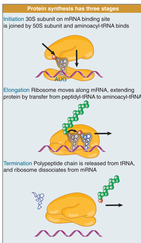
FIGURE 8.7 Protein synthesis falls into three stages.
