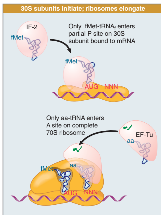
FIGURE 8.14 Only fMet-tRNA f can be used for initiation by 30S subunits; other aminoacyl-tRNAs ( \alpha\alpha -tRNA) must be used for elongation by 70S ribosomes.
