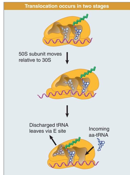
FIGURE 8.29 Models for translocation involve two stages. First, at peptide bond formation the aminoacyl end of the tRNA in the A site becomes relocated in the P site. Second, the anticodon end of the tRNA becomes relocated in the P site.
