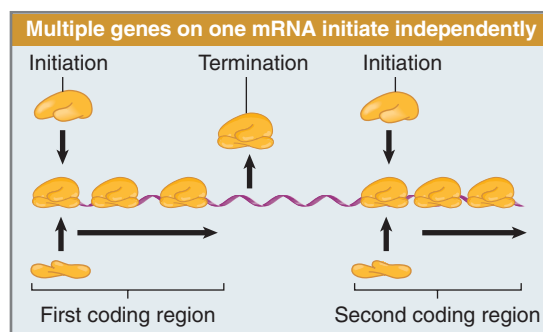
FIGURE 8.17 Initiation occurs independently at each cistron in a polycistronic mRNA. When the intercistronic region is longer than the span of the ribosome, dissociation at the termination site is followed by independent reinitiation at the next cistron.
